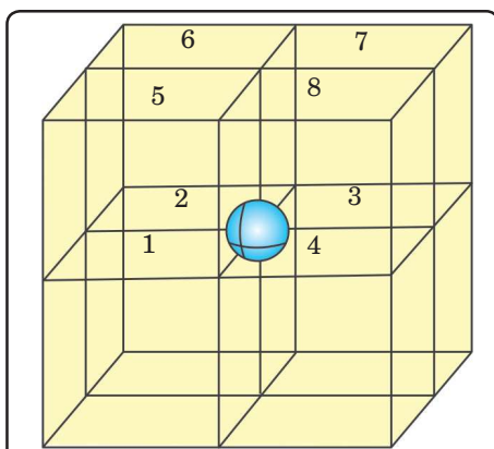
Fig. 15. A corner atom in cubic unit cell is shared by 8 unit cells.
