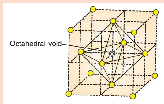
(a) Octahedral void at body centre of ccp unit cell
