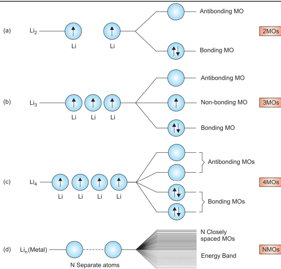
Fig. 49. Formation of molecular orbitals from 2, 3, 4 and N lithium atoms.
