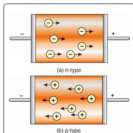
Fig. 58. Conduction in n-type and p-type of semiconductors.
