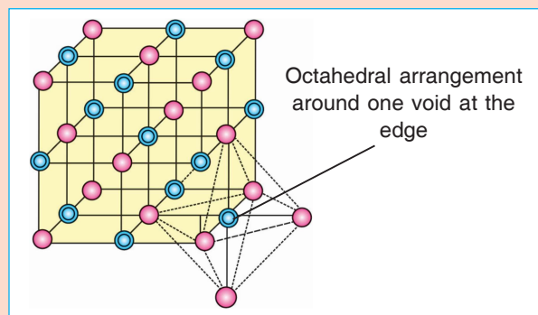
(b) 12 octahedral voids at the edges in ccp unit cell (shown ●)
