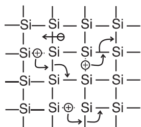
(b) Intrinsic semi-conduction in silicon
