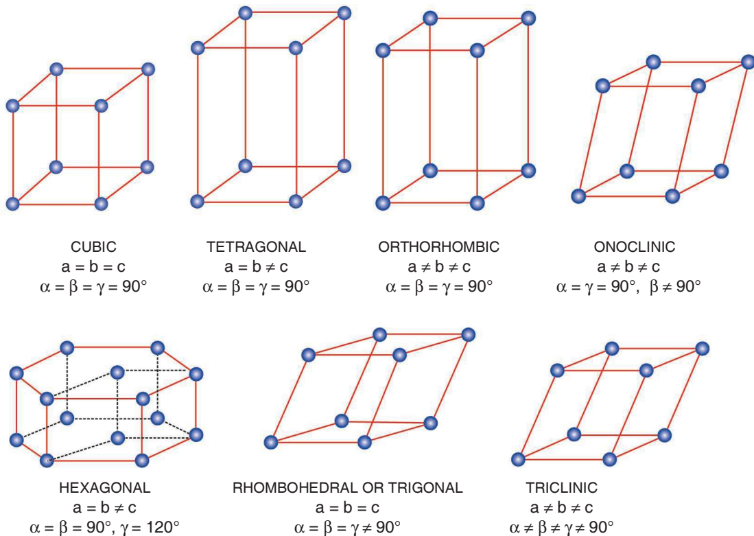
Fig. 12. The seven crystal systems.
