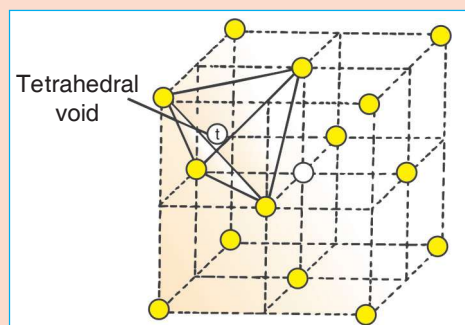
(a) One tetrahedral void in ccp structure.
