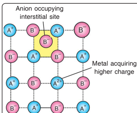
Fig. 47. Metal deficient defect due to extra anion.
