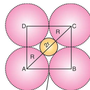
Octahedral void with radius r
