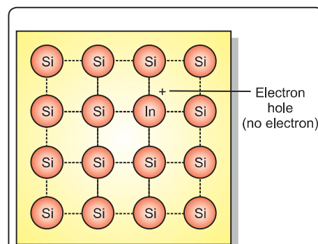
Fig. 57. Indium doped silicon semiconductor.
