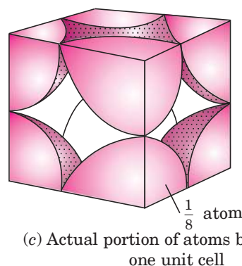
Fig. 18. Simple cubic arrangement and number of spheres per unit cell.
