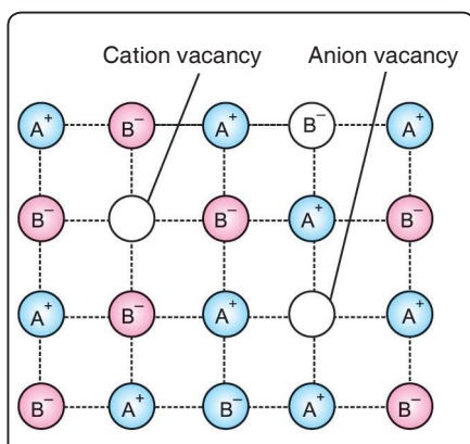
Fig. 42. The Schottky defect in crystals.
