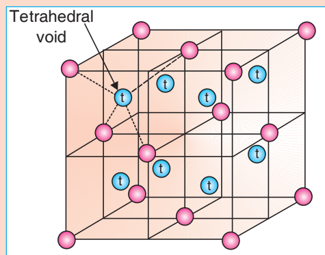
(b) Eight tetrahedral voids in ccp structure.
