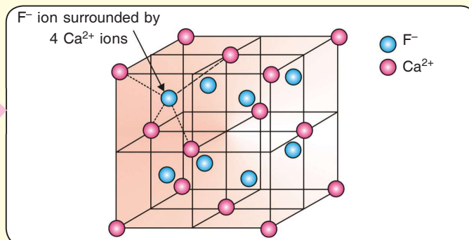
Calcium fluoride (CaF 2 )
