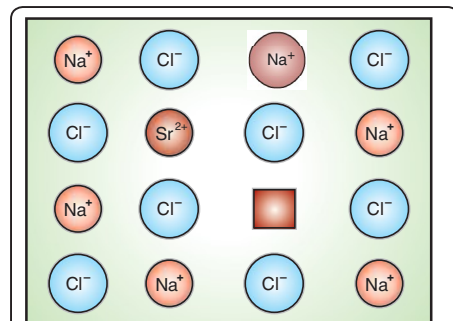
Fig. 48. Introduction of a cation vacancy in NaCl by substitution of Na^+ by Sr^{2+} .
