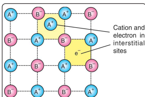
Fig. 45. Metal excess defects due to extra cation.
