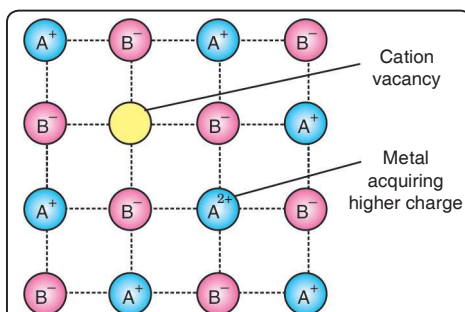
Fig. 46. Metal deficient defect due to cation vacancy.
