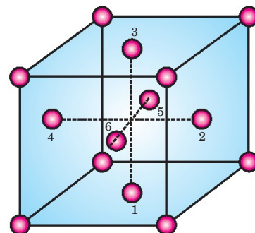
(c) Face centred cubic: Atoms at the corners and centre of each face. Atoms 1, 2, 3, 4, 5, and 6 are present at the centres of six faces (atom 5 corresponds to atom at the centre of back face and atom 6 corresponds to the centre of front face.)
